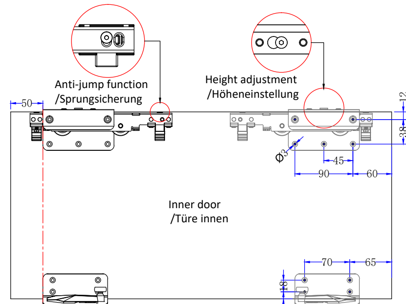
Adjustment according to door thickness /Einstellung dicke Türen
