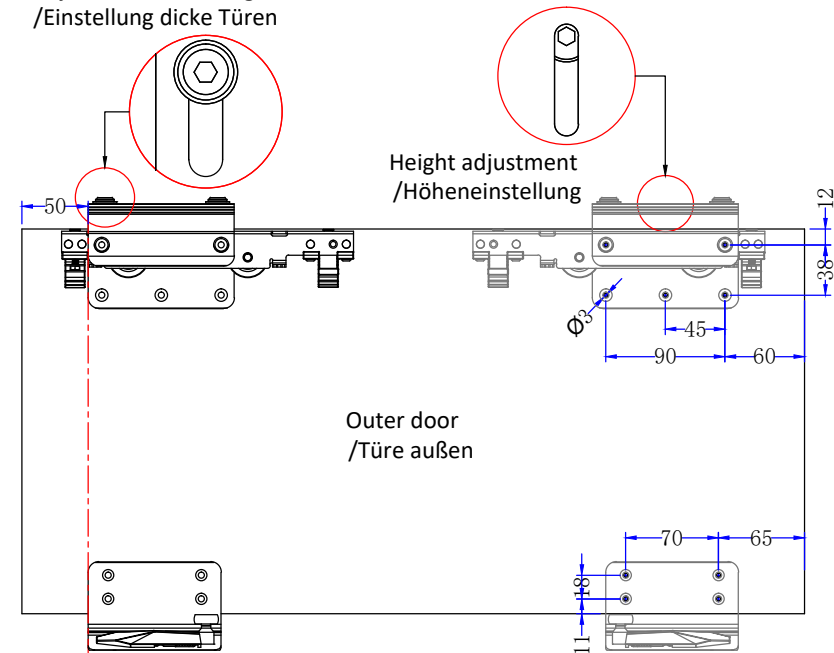
Adjustment according to door thickness /Einstellung dicke Türen
